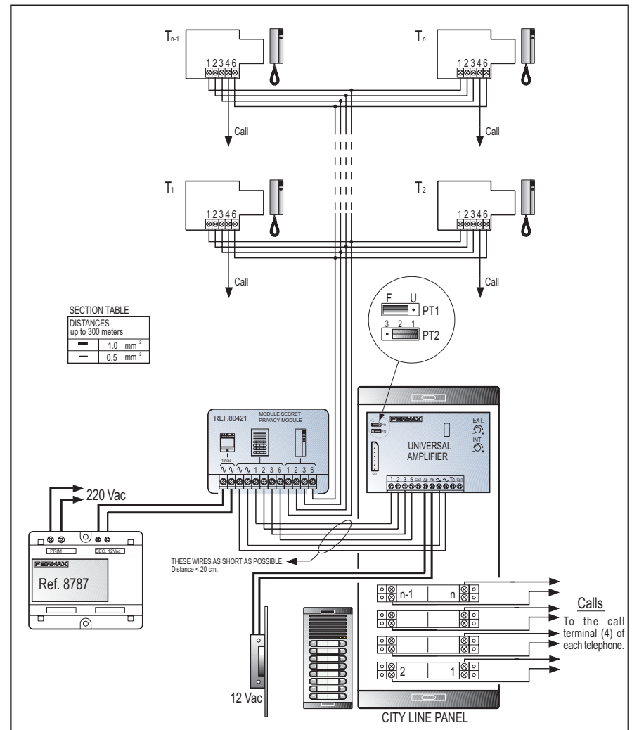
WIRING DIAGRAM
